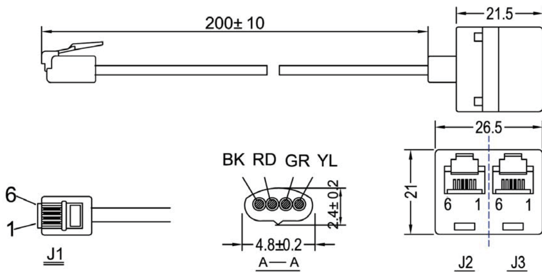
Wiring Connection
