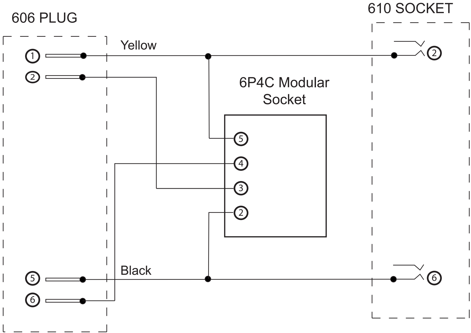
P6163IVO Wiring Diagram (Mode 3)
