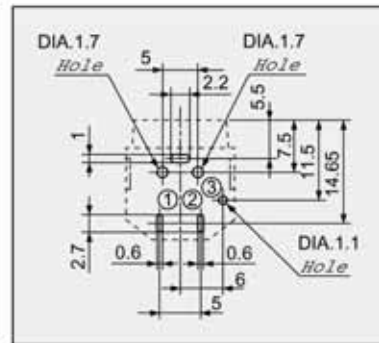
PCB Footprint
